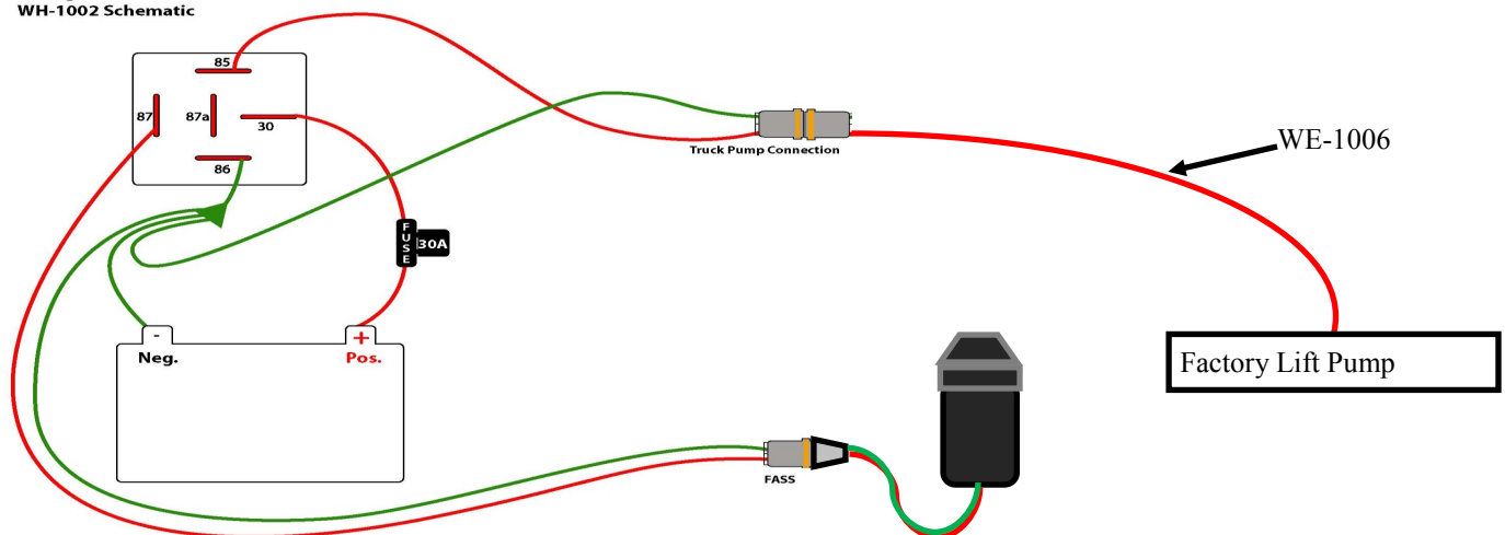
FASS Wiring Harness WH-1002 Schematic
